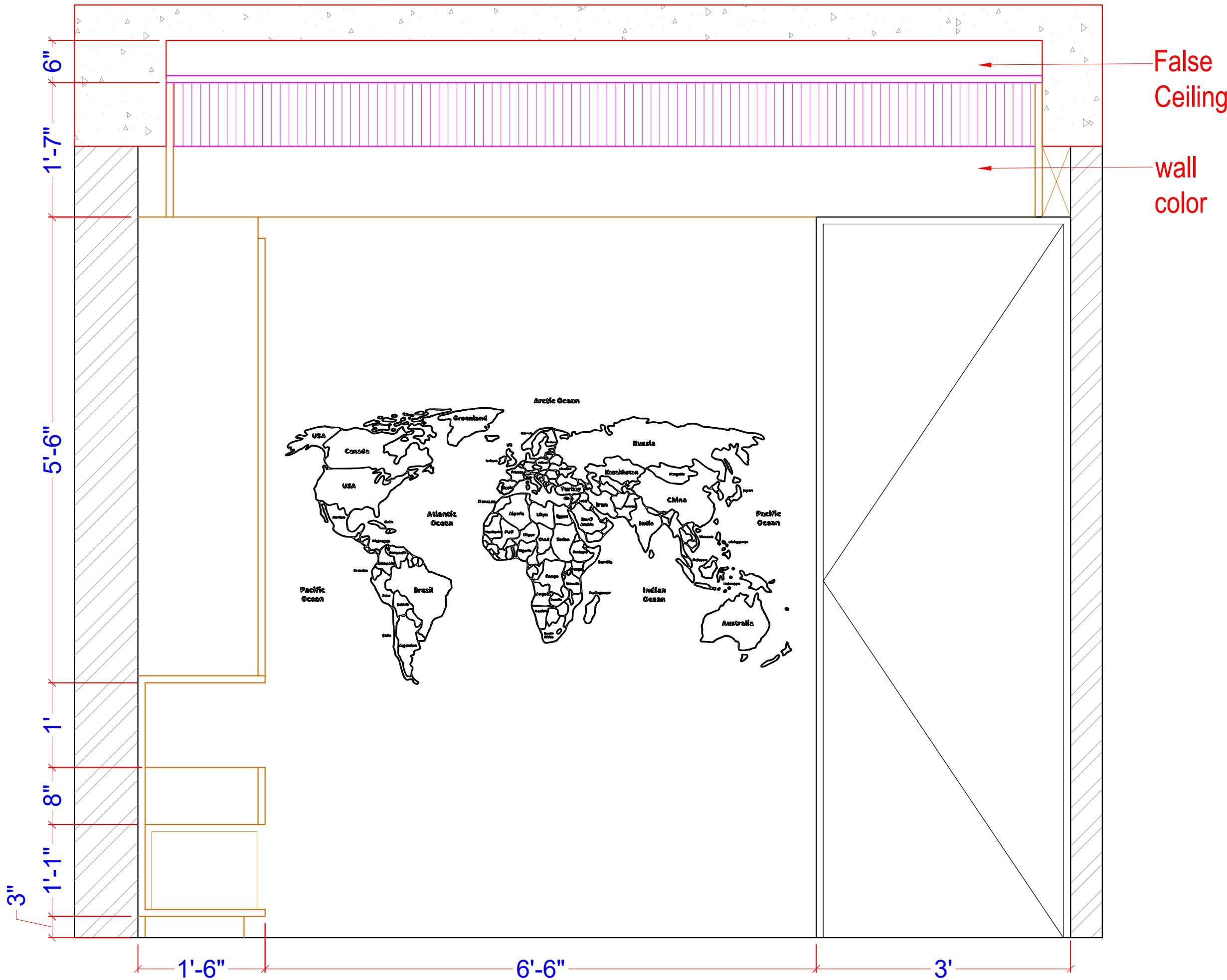
WALL ELEVATION - D
